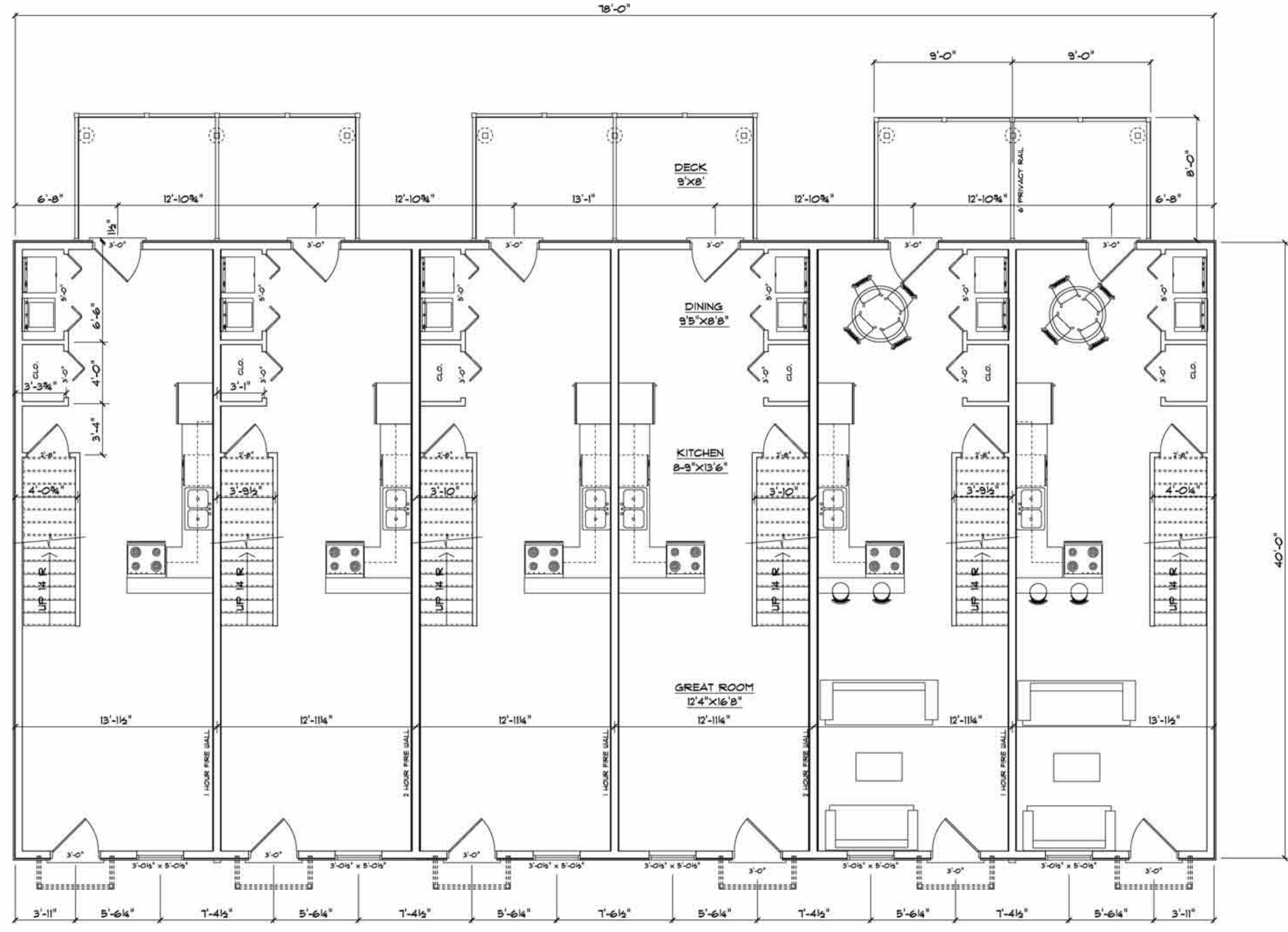
FLOOR PLAN
